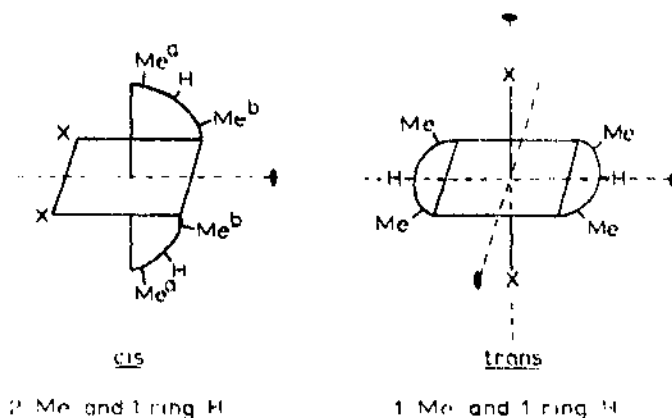
Fig. 1. \text{M}(\text{acac})_2\text{X}_2 cis and trans isomers. The methyl groups in the a and b sites of the polar cis isomer ( \text{C}_2 symmetry) are inequivalent. All methyl groups in the non-polar trans isomer ( \text{D}_{2h} symmetry) are equivalent. (Reproduced with permission from Ref. [9].)
