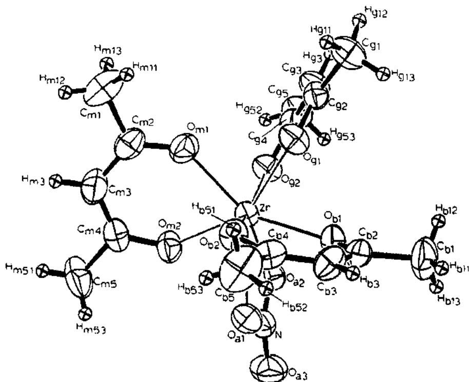
Fig. 9. Dodecahedral structure of the Zr(acac)_3(NO_3) molecule. The ligands are labeled a , b , m , or g according to the dodecahedral edge that the ligand spans. (Reproduced with permission from Ref. [43].)
