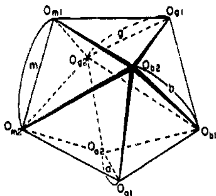
Fig. 10. Ligand wrapping pattern in Zr(acac)_3(NO_3) . The ligands are labeled a , b , m , or g according to the dodecahedral edge that the ligand spans. (Reproduced with permission from Ref. [43].)
